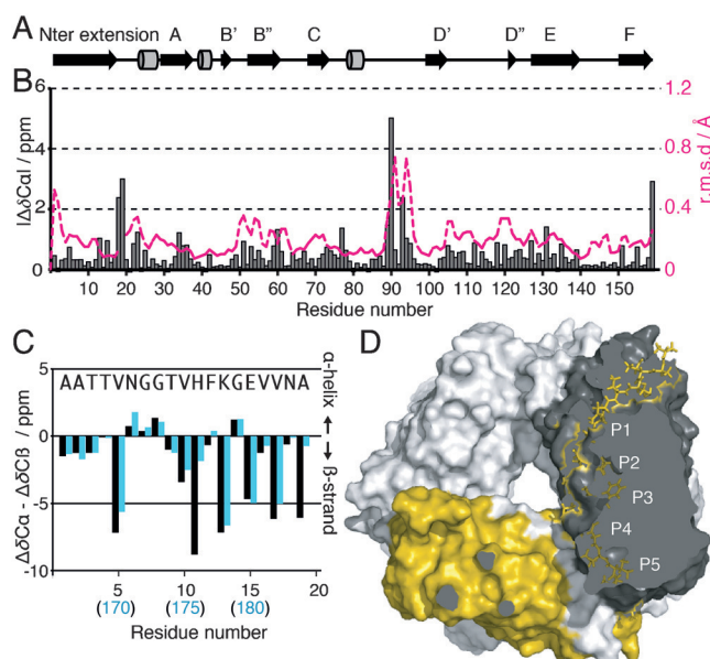
Figure 2. A) Secondary structure of the type 1 FimA pilus. B) ^{13}\text{C} chemical-shift differences between the solution NMR data of self-complemented FimA monomers [11] and ssNMR chemical shifts of wt FimA pili (absolute values of \Delta(\text{solution NMR} - \text{ssNMR})\delta\text{C}\alpha ). The dashed pink line indicates the backbone r.m.s.d. of the solution NMR structure of the self-complemented FimA monomer (PDB entry 2JTY). Residues A1–N18 in 2JTY have been replaced with residues A166–N183 representing the donor strand in 2JTY. The r.m.s.d. for the connecting residue A19 has been discarded because it is found in different environments in the monomeric construct FimAa and the FimA pili. C) Secondary structure of the FimA donor strand, as determined by secondary chemical shifts ( \Delta\delta\text{C}\alpha - \Delta\delta\text{C}\beta ), compared for the assembled pilus (black) and the self-complemented FimAa construct (cyan). Negative values ( >3 in a row) indicate \beta -strand conformation. D) Surface view of a FimA pilus cut at the level of subunits i-1 (yellow) and i (gray). The donor strand of subunit i-1 is detailed in a stick representation. For clarity, subunits i-2 to i-5 are depicted in white, and the donor strand of subunit i is omitted.
